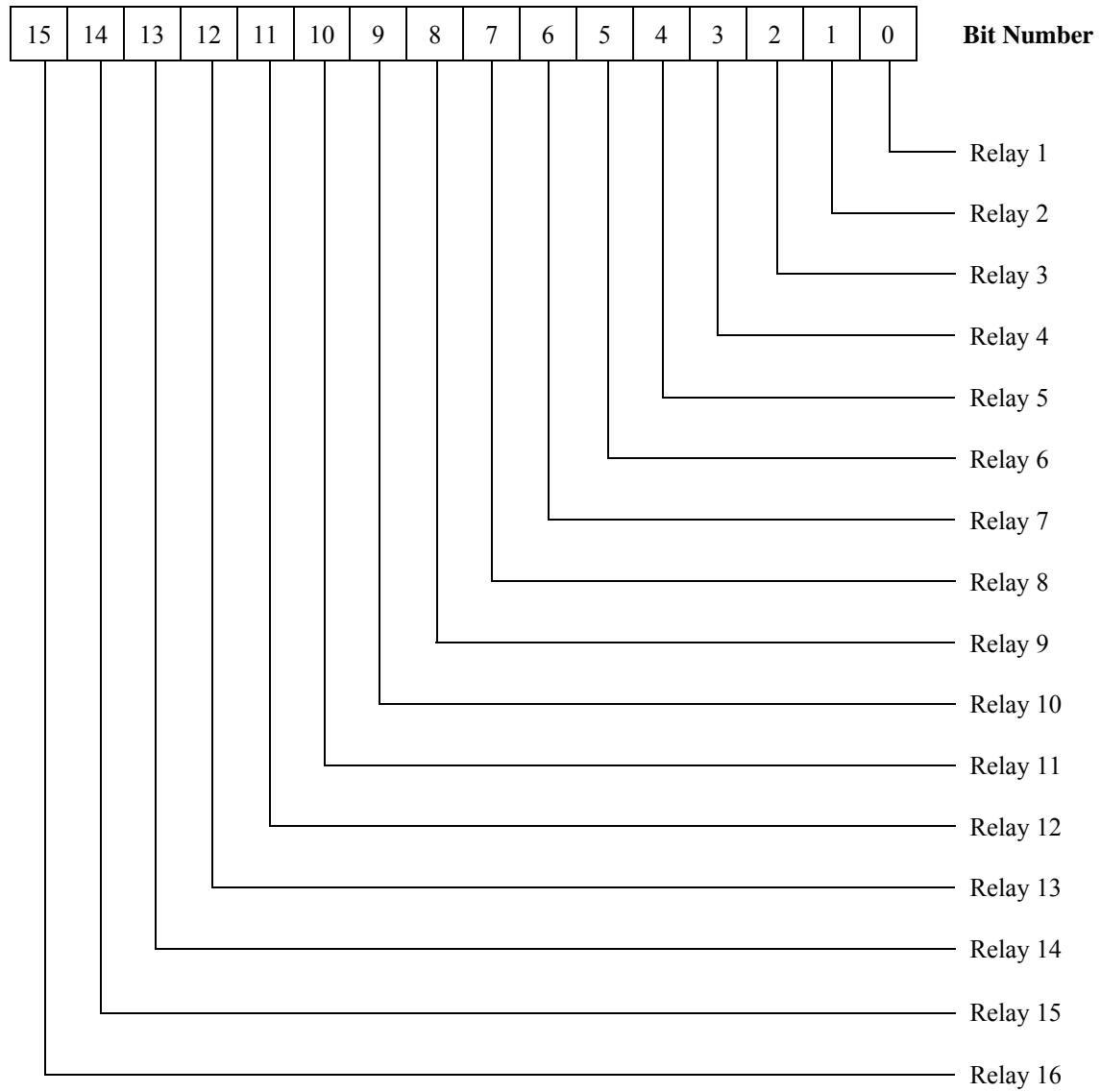
FIGURE 3-1: RELAY REGISTER
