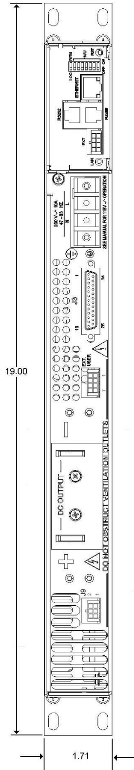
Figure 3. Rear View – Ethernet
